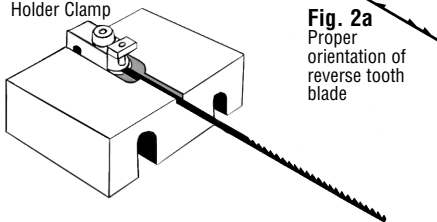
Fig. 2 Fixture Block
