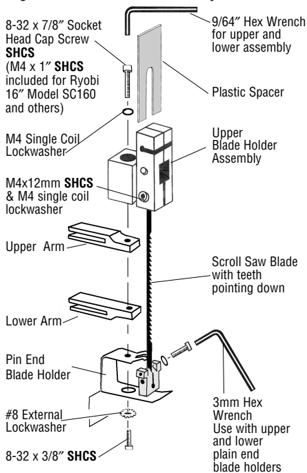
Fig. 1 Plain End Blade Assembly
